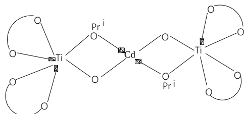
Figure 5: Suggested structure of [\text{CdO}_2\text{Ti}_2(\text{OPr}^i)_2(\text{L})_4]
