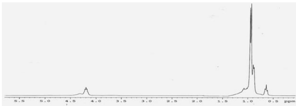
Figure 1: ^1\text{H} NMR spectrum of [\text{CdO}_2\text{Ti}_2(\text{OPr}^i)_6]
