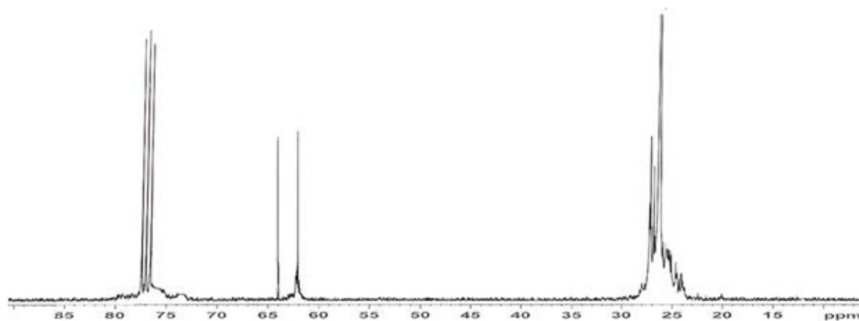
Figure 2: ^{13}\text{C} NMR spectrum of \text{CdO}_2\text{Ti}_2(\text{OPr}^i)_6
