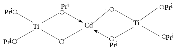
Figure 4: Suggested structure of [\text{CdO}_2\text{Ti}_2(\text{OPr}^i)_6]
