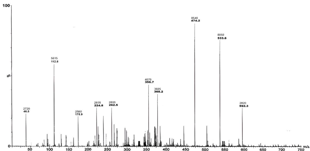
Figure 3: Mass spectrum of \text{CdO}_2\text{Ti}_2(\text{OPr}^i)_6
